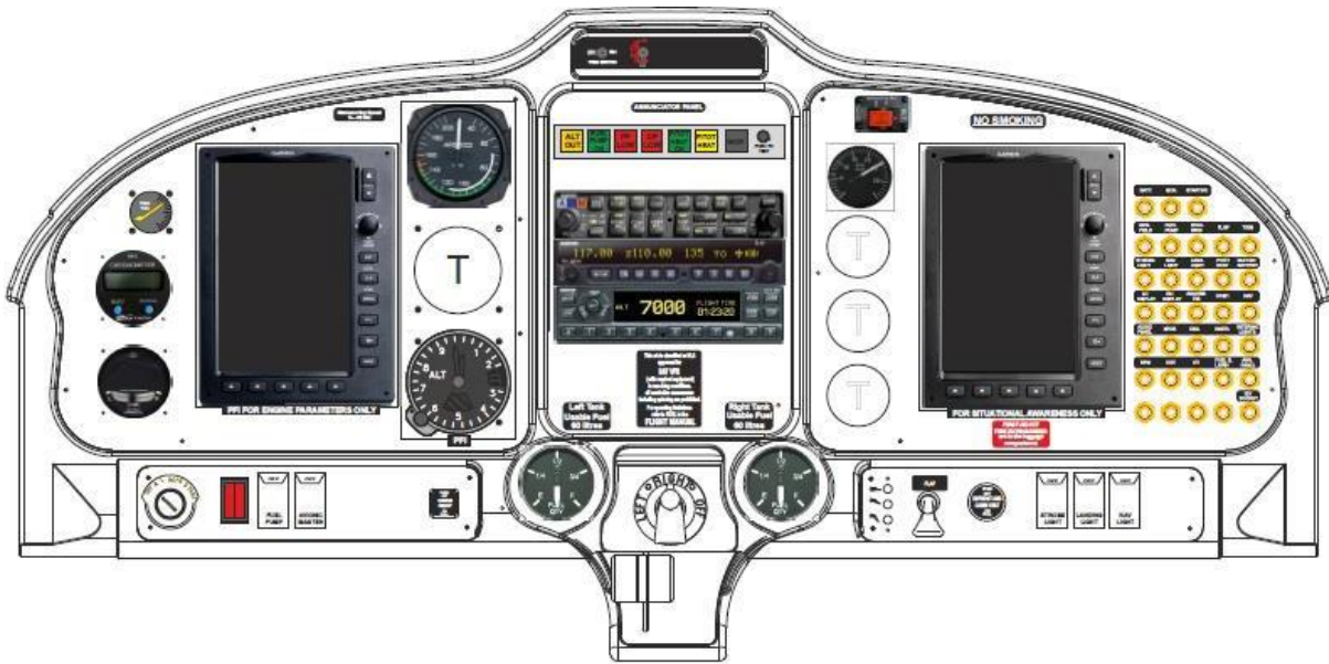
Fig. 7-5. INSTRUMENT PANEL
